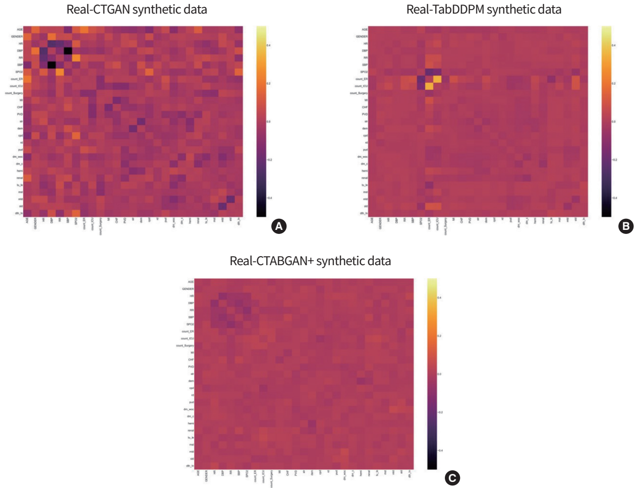
Supplementary Fig. 2. Comparison of correlation values between real and synthetic data with (A) conditional tabular generative adversarial network (CTGAN), (B) tabular denoising diffusion probabilistic model (TabDDPM), and (C) conditional tabular generative adversarial network + (CTABGAN+).
